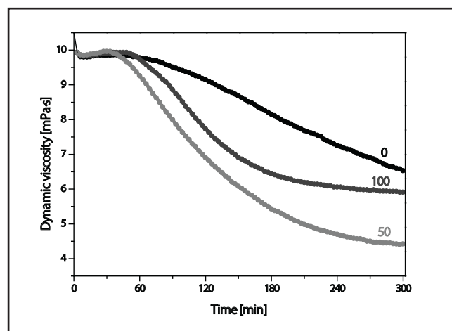
Fig. 2. Time dependent HA degradation by the oxidative system 1.0 µM CuCl 2 and 100 µM ascorbate (0). Effect of the addition of D-pen at the concentrations 50 or 100 µM before the reaction onset.
