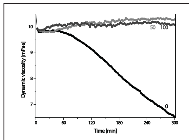
Fig. 3. Time dependent HA degradation by the oxidative system 1.0 µM CuCl 2 and 100 µM ascorbate (0). Effect of the addition of L-GSH at the concentrations 50 or 100 µM before the reaction onset.
