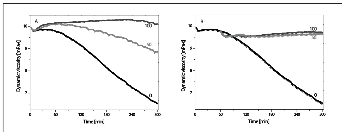
Fig. 4. Time dependent HA degradation by the oxidative system 1.0 \mu\text{M} \text{CuCl}_2 and 100 \mu\text{M} ascorbate (0). Effect of the addition of cysteamine (50, 100 \mu\text{M} ) before the reaction onset (A) or 1 h after the reaction onset (B).
